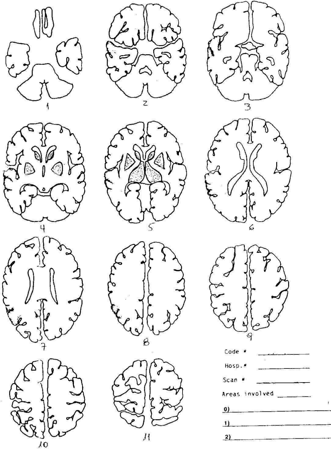
Fig. 4. Plotting of the lesion seen in Fig. 3, in its best-fitting template system.
